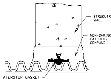
WATERSTOP GASKET
